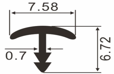
INLAY HALF ROUND PROFILE (6T1)
