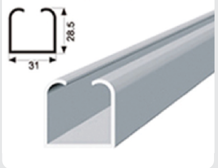
C CHANNEL PROFILE FOR 8 1/4 WHEEL ROLLER
